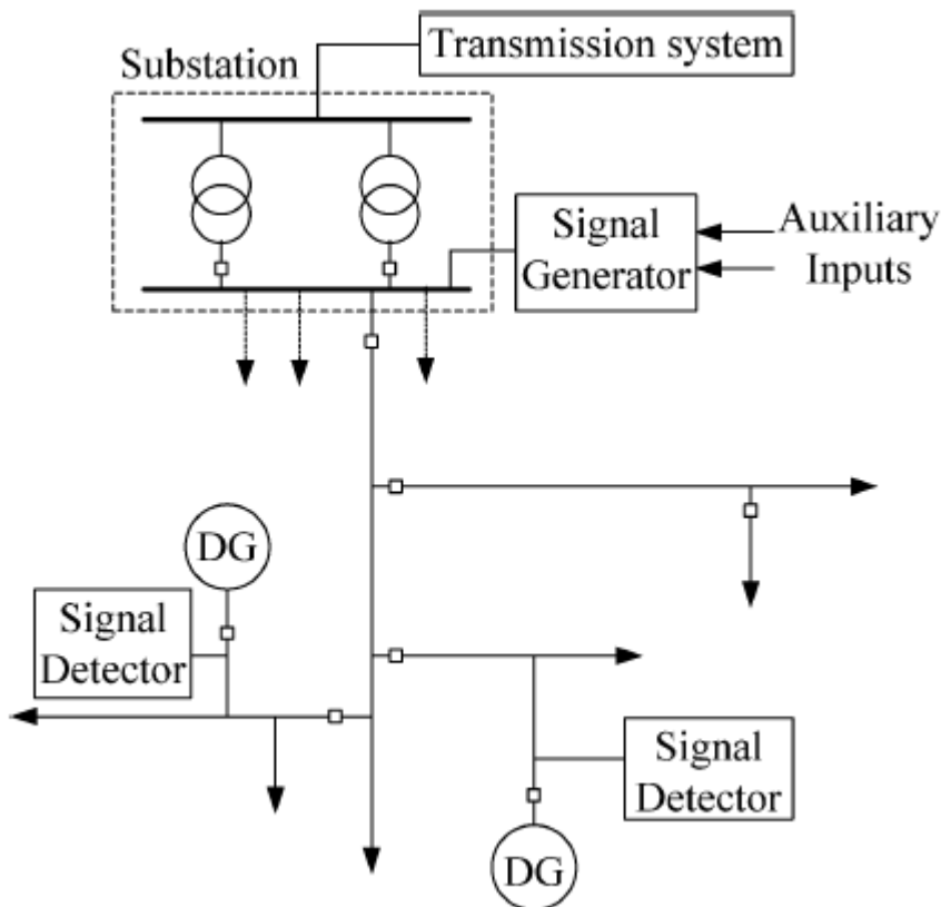
Fig. 1. Illustration for the proposed anti-islanding scheme.
