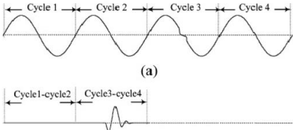
Fig. 2 Subtraction Pattern for signal Extraction
