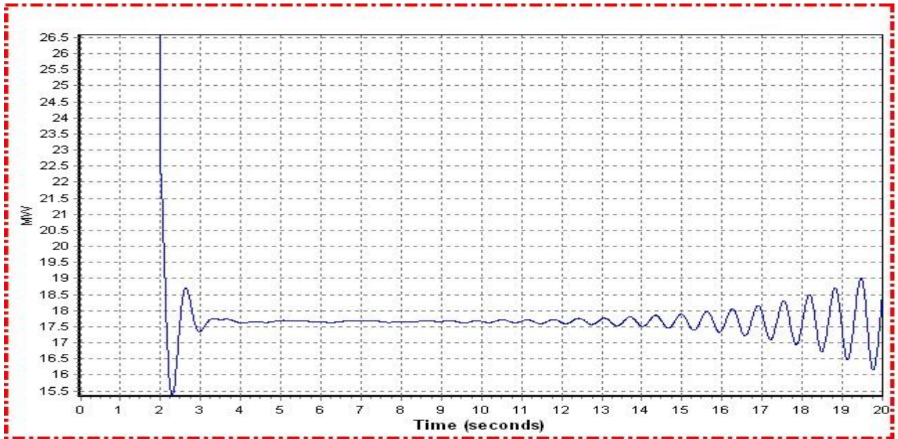
Fig.4 active power during tripping
